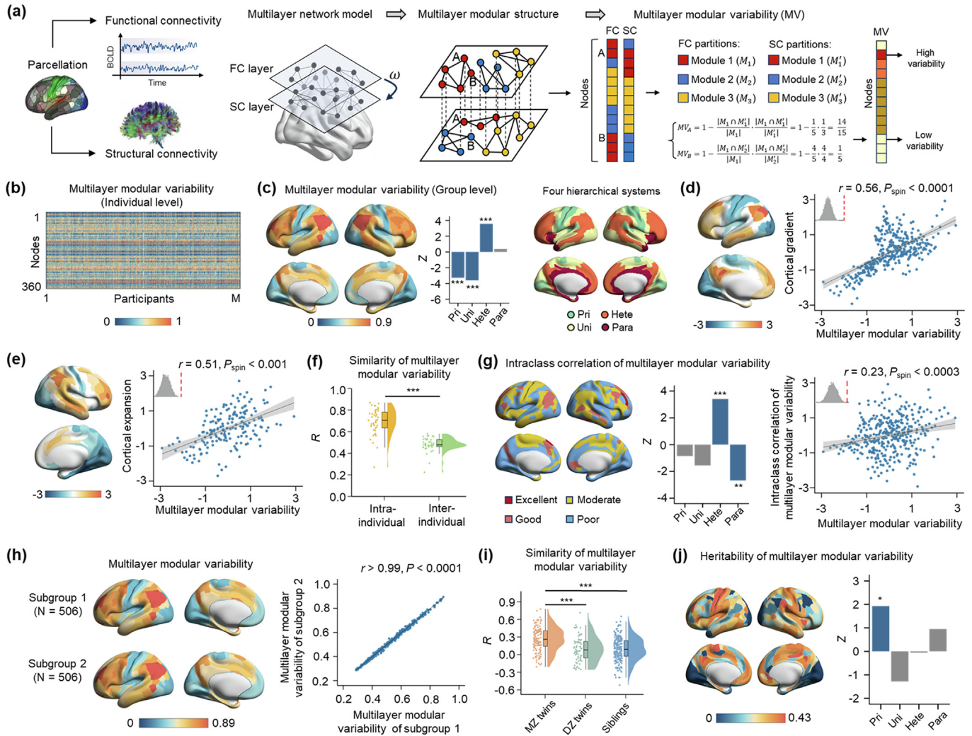
Fig. 1. Spatial topography and its test–retest reliability and heritability of multilayer modular variability in the interdependent SC-FC connectome. (a) Schematic of SC-FC connectome construction and multilayer modular variability (MV) calculation. (b) Multilayer modular variability at individual-level. (c) The spatial topography of group-level multilayer modular variability and its correlations with the functional connectivity gradient (d) and evolutionary expansion of cortical surface area (e). (f) Similarity of multilayer modular variability of intra-individual and inter-individual. (g) Spatial topography of intraclass correlation and its correlation with multilayer modular variability. (h) Correlation of multilayer modular variability between two half-split subgroups. (i) Similarity of multilayer modular variability among monozygotic, dizygotic and siblings pairs. (j) Spatial distribution of multilayer modular variability heritability. Bar plots show values in four hierarchical systems, with colored bars indicating cortical systems differing from null model. In scatter plots, gray shading represents 95% confidence interval, upper-left histograms show null-model r values, and red dotted lines indicate empirical r values. Each dot represents the mean value of node across participants. To better visualize the scatter plots, the raw values were scaled using a rank-based inverse Gaussian transformation. Pri: primary cortex; Uni: unimodal cortex; Hete: heteromodal cortex; Para: paralimbic cortex. MZ: monozygotic; DZ: dizygotic. * P < 0.05 , ** P < 0.01 , *** P < 0.001 .
