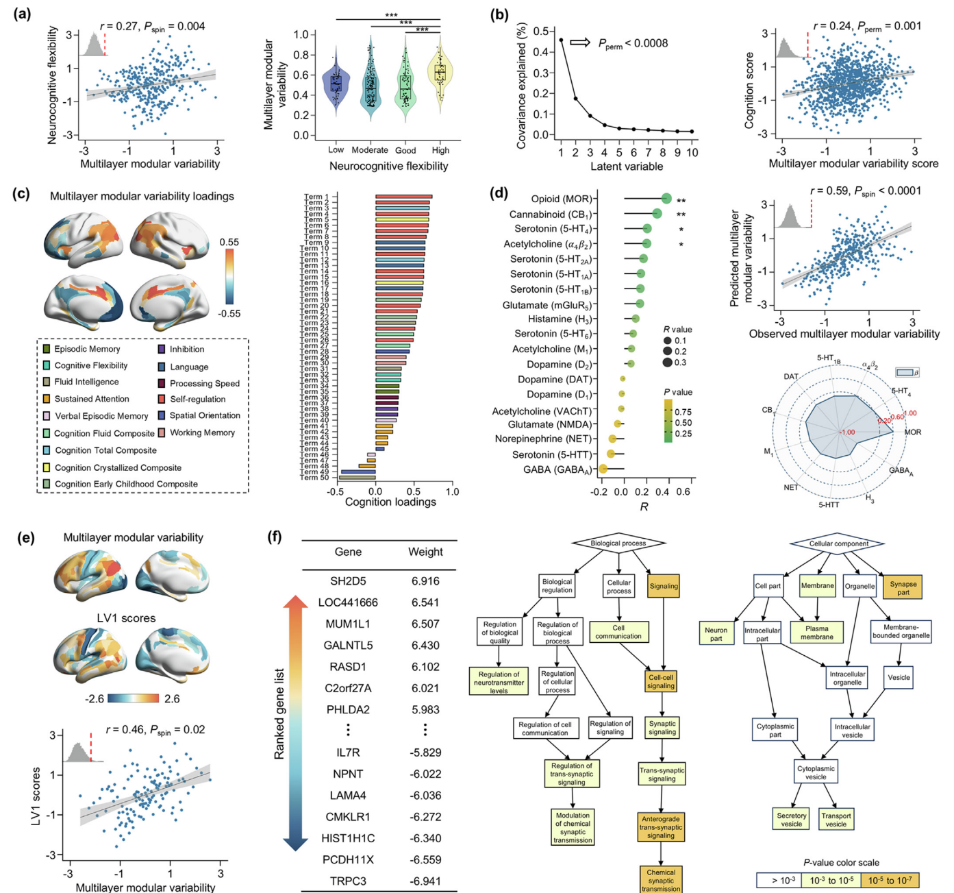
Fig. 2. Cognitive and molecular associations of multilayer modular variability in the interdependent SC-FC connectome. (a) Correlation between multilayer modular variability and neurocognitive flexibility, shown via violin plot for nodes with low to high flexibility. (b) Partial least squares (PLS) analysis between individual multilayer modular variability and cognitive measures. First PLS latent variable (LV1) shows optimal linear combination of brain regions covarying with cognitive scores (46% covariance explained). For LV1, the multilayer modular variability score and cognition score were correlated. Detailed methods are presented in Supplementary Methods 2.8 . (c) Significant loadings of brain regions and cognition terms (1000 bootstrap repetitions). Cognitive processes shown in left panel's dashed box with color coding. Full cognitive details in Table S2 (online). (d) Left panel depicts the correlation between receptors/transporters and multilayer modular variability. Scatter plot shows the prediction results of the elastic net regression. Radar Chart displays significant predictive features with regression coefficients ( \beta ). (e) Multivariate PLS regression analysis between group-level multilayer modular variability and gene expression. LV1 component captures dominant covariation between regional modular variability and transcriptomic patterns, showing a significant correlation with multilayer modular variability. Detailed methods are presented in Supplementary Methods 2.10 . (f) Gene ontology enrichment analysis results from gene list (details in Table S3 (online)). Each dot in scatter plots of (a), (d) and (e) represents the mean value of node across participants. In scatter plot of (b), dots represent individual participant scores on the latent components of brain and cognitive measurements.
